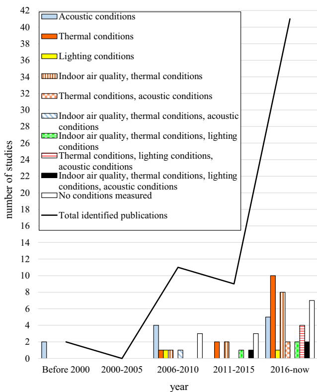
FIGURE 3 The number of studies addressing the IEQ in classrooms in higher education, the distribution over the indoor environmental parameters, and the distribution over the years
